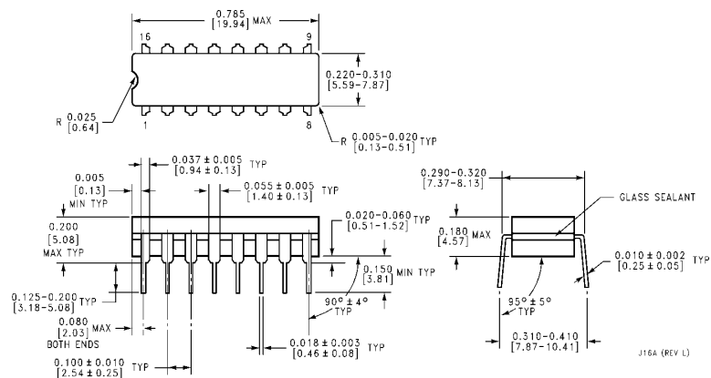
16-Lead Ceramic Dual-In-Line Package (J) Order Number DM54LS47J NS Package Number J16A
