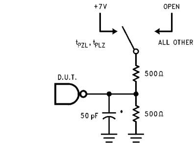
*Includes jig and probe capacitance FIGURE 1. Test Load
